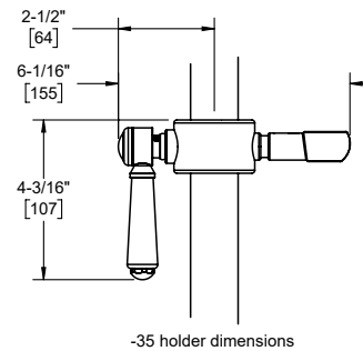
-35 holder dimensions
