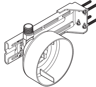
Body Spray Rough-In
