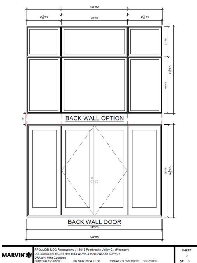
MARVIN WINDOW SCHEMATIC FOR NEW WINDOWS
