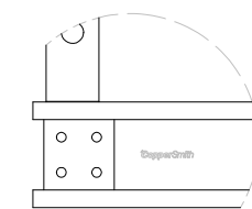
APRON DETAIL SCALE 1 / 6
